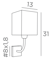
Lampshade ABA 1 # # 13-13-15 cm Lampshade code : 1300 + fabric code ↳ 18,5 cm
